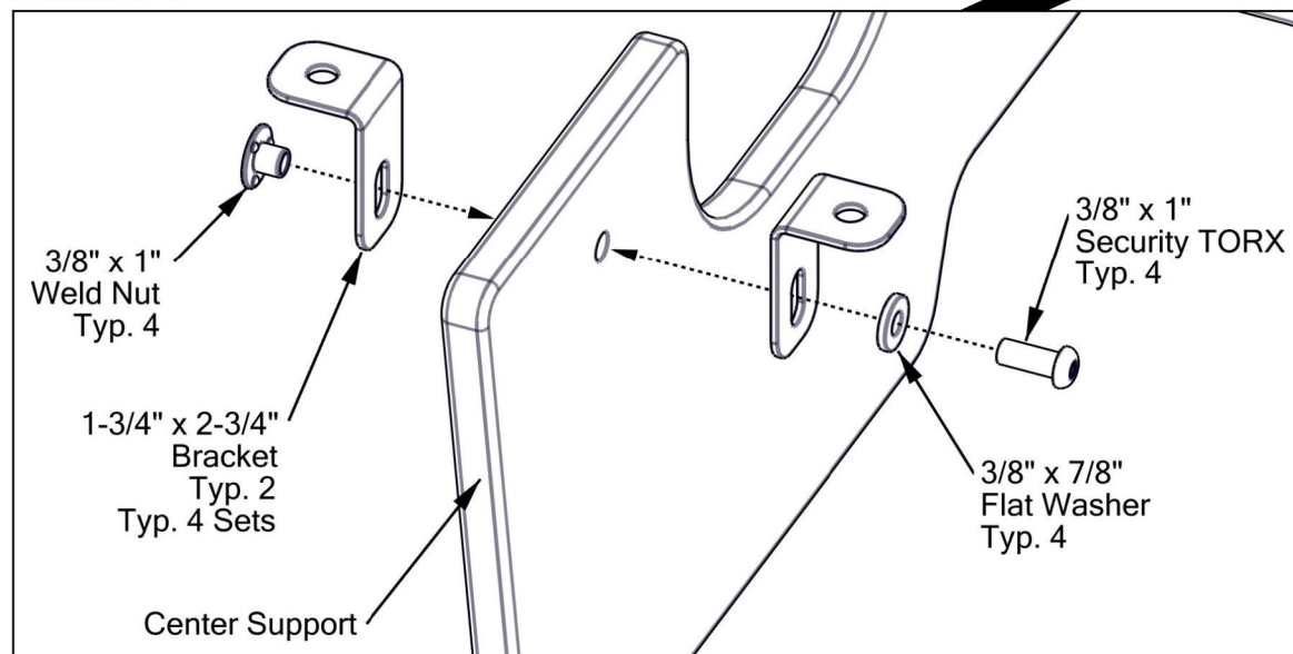
Detail 2-1
