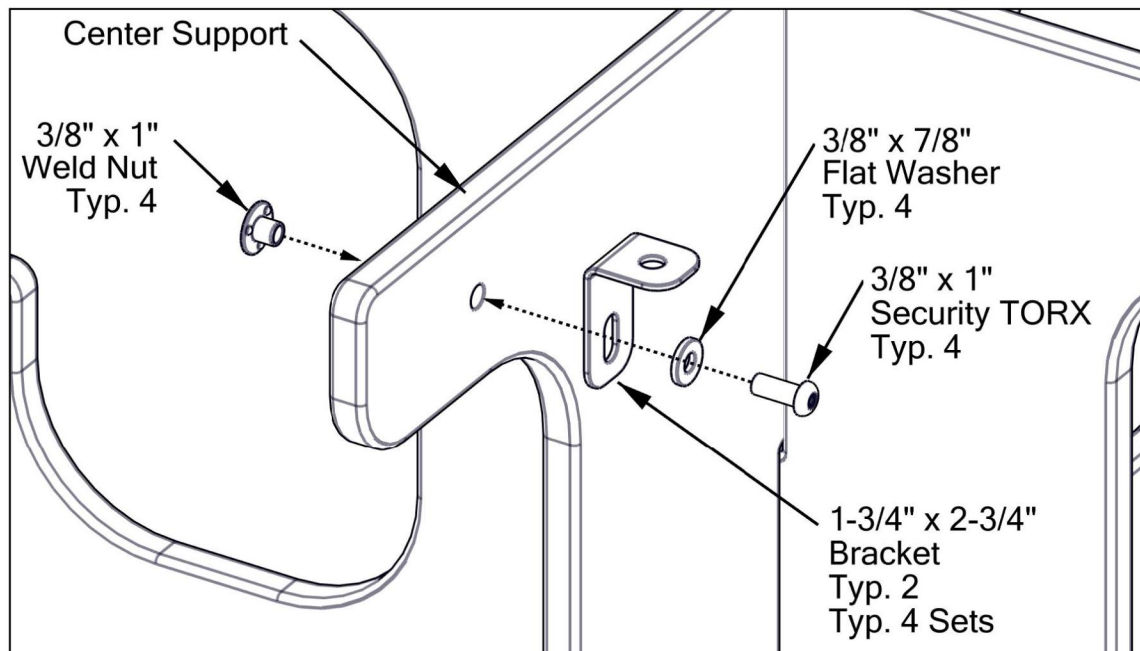
Detail 3-1
