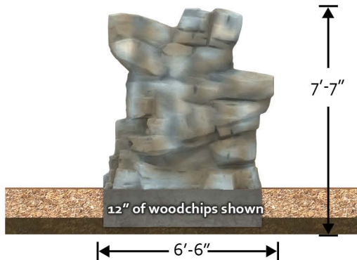
12" of woodchips plus 3" of fill over footing, or: 15" total of fill and synthetic playground safety surfacing over footing.
